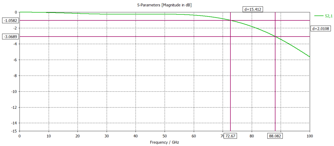
Figure 2: Simulated Insertion loss S21
