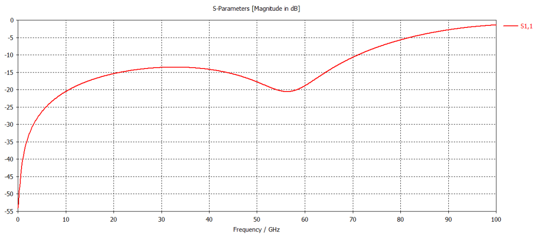
Figure 3: Simulated Return Loss S11
