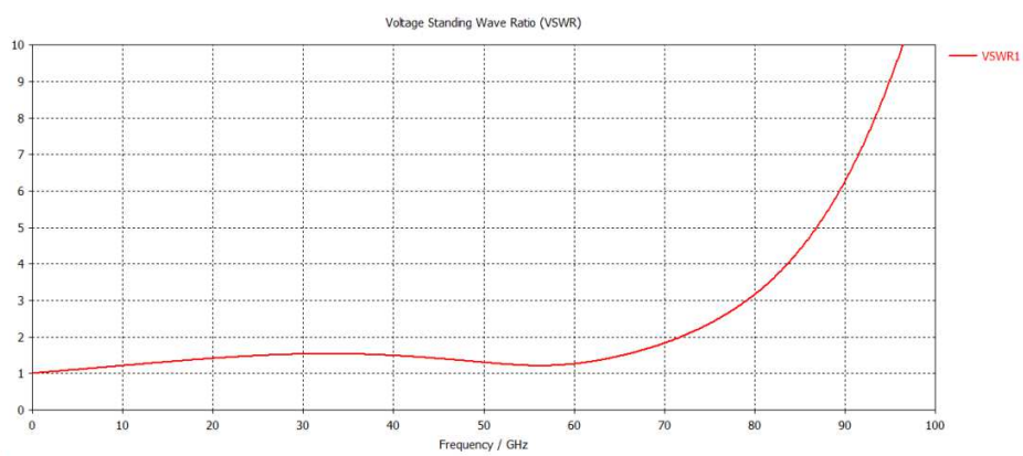
Figure 5: Simulated VSWR
