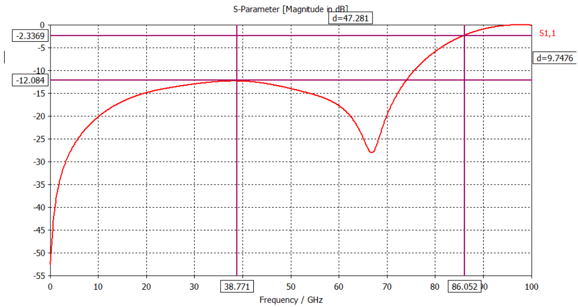
Figure 3: Simulated Return Loss S1,1
