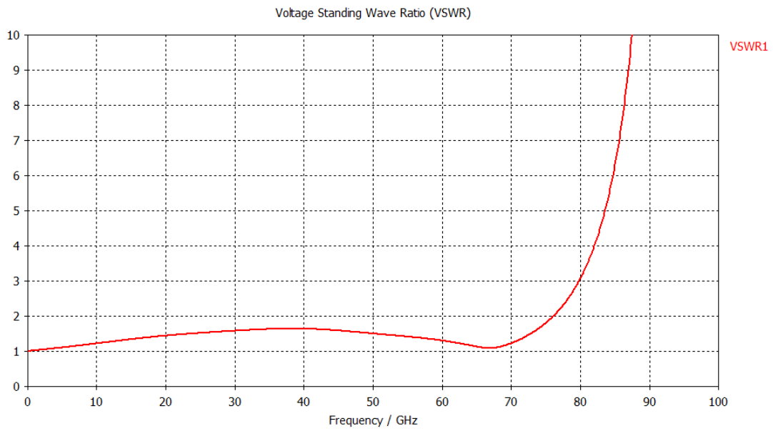
Figure 5: VSWR
