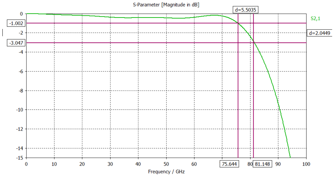
Figure 2: Simulated Insertion loss: -1dB at > 75.6 GHz (minimum bandwidth across the array).
