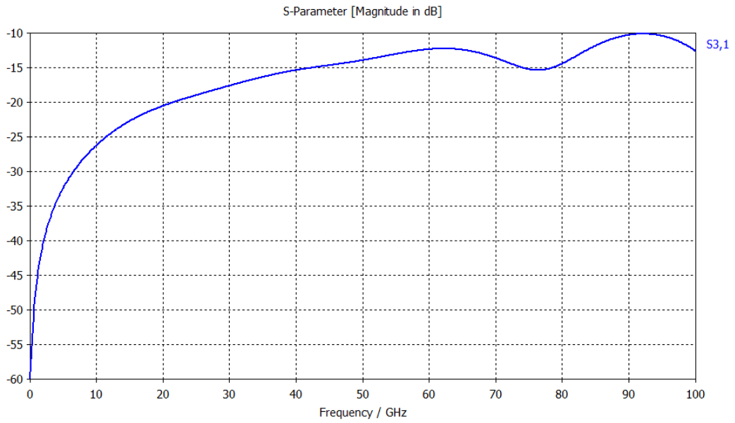
Figure 4: Crosstalk. S31
