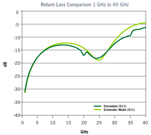
Figure 6. GSG P2A Return Loss, 0.8 mm pitch
