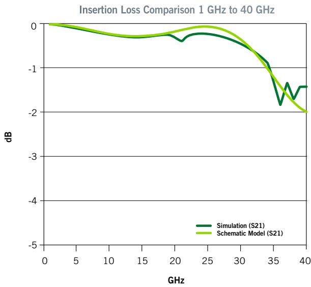
Figure 5. GSG P2A Insertion Loss, 0.8 mm pitch
