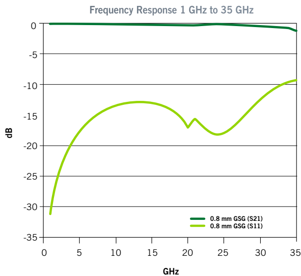
Figure 2. GSG P2A Insertion Loss and Return Loss, 0.8 mm pitch
