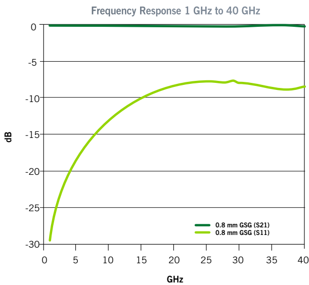
Figure 9. GSG P8A Insertion Loss and Return loss, 0.8 mm pitch
