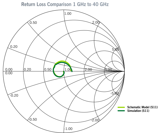
Figure 14. GSG P8A Return Loss plotted on Smith chart, 0.8 mm pitch
