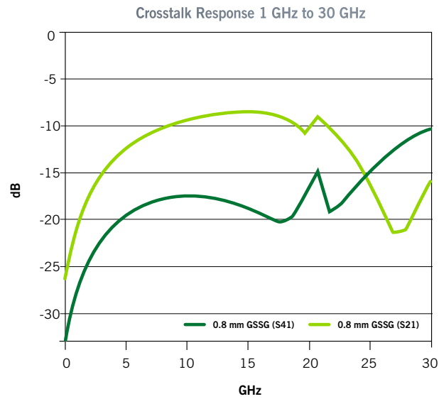
Figure 16. GSSG Crosstalk Response, 0.8 mm pitch
