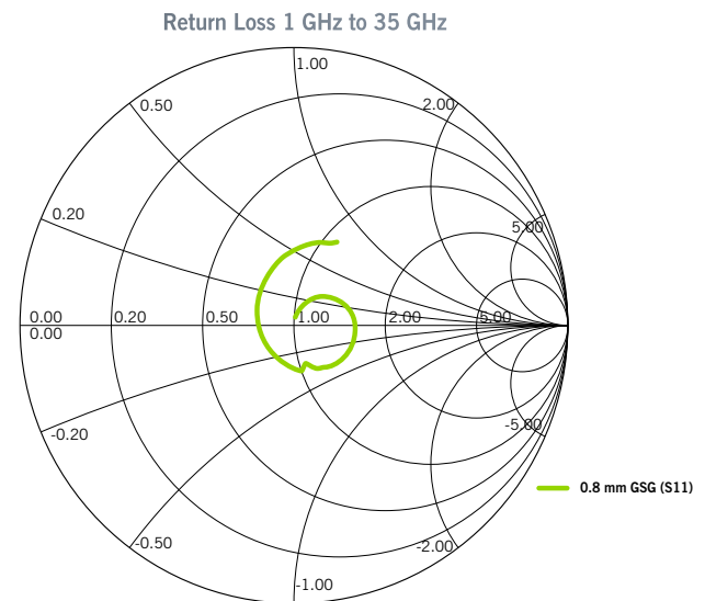
Figure 3. GSG P2A Return Loss plotted on Smith chart, 0.8 mm pitch
