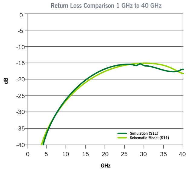
Figure 13. GSG P8A Return Loss, 0.8 mm pitch
