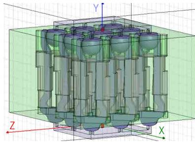
Figure 8. 0.8 mm GSG P8A model configuration
