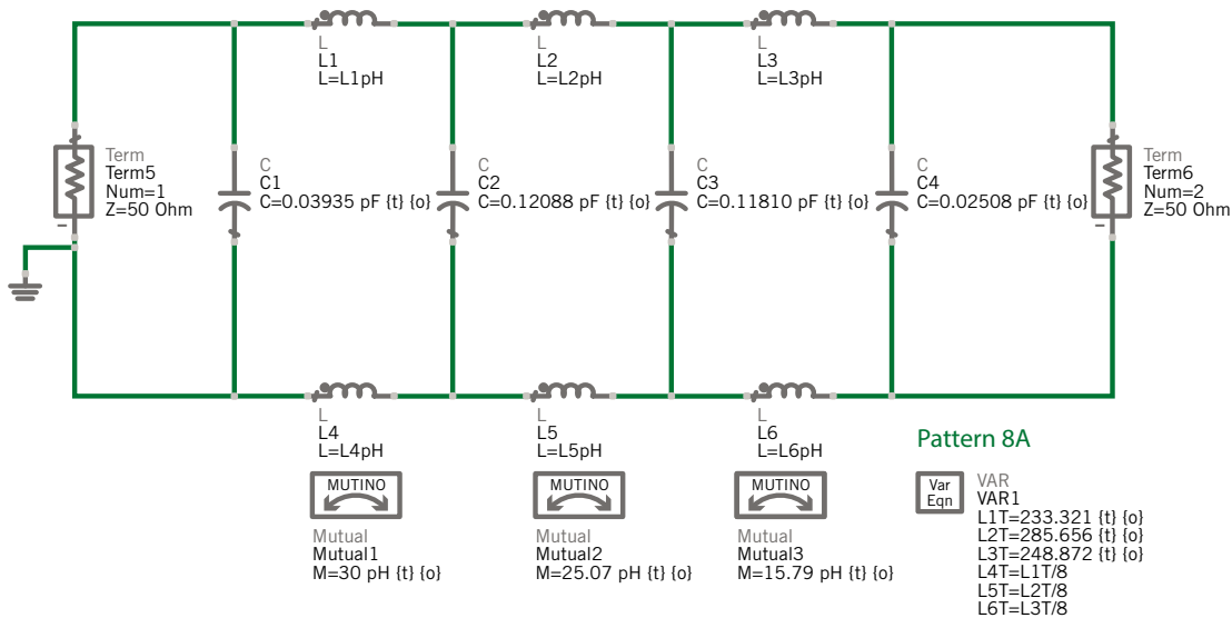
Figure 11. GSG P8A Schematic Model, 0.8 mm pitch
