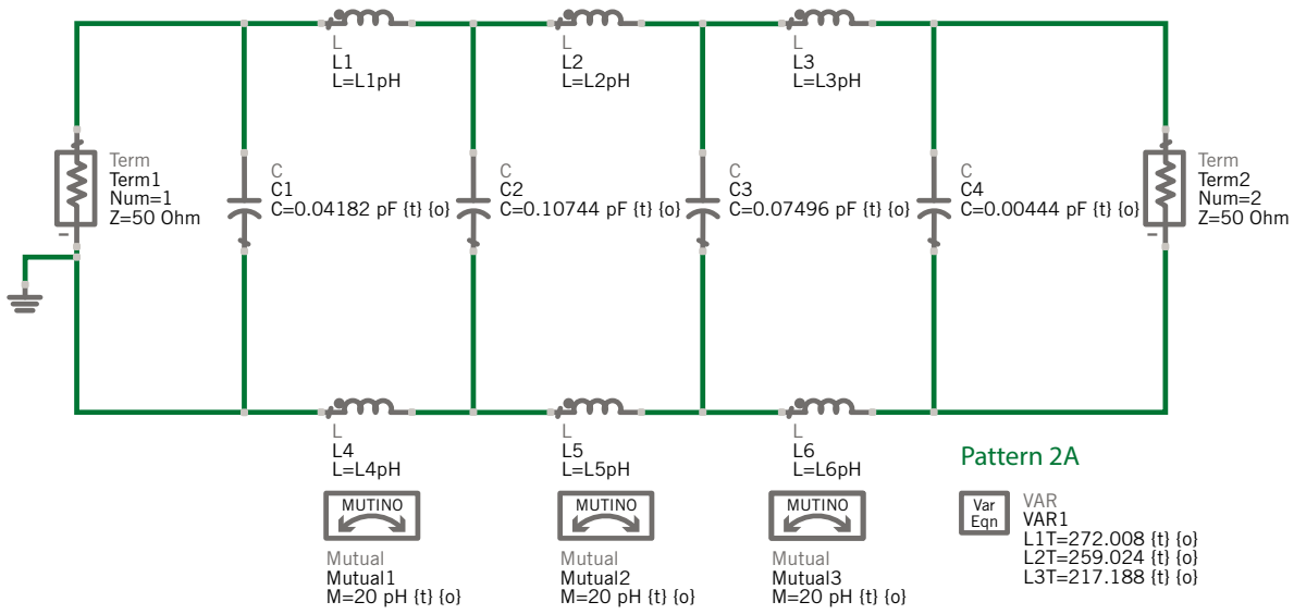
Figure 4. GSG P2A Schematic Model, 0.8 mm pitch
