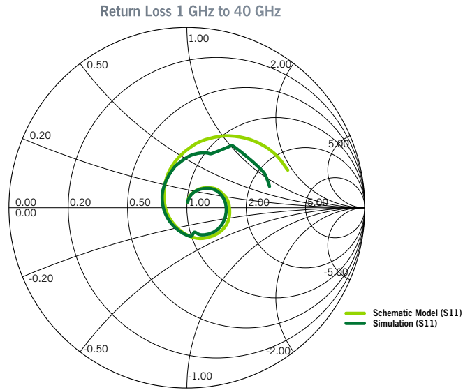
Figure 7. GSG P2A Return Loss plotted on Smith chart, 0.8 mm pitch
