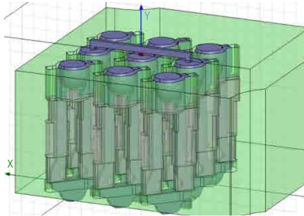
Figure 1. 1.0 mm GSG P2A model configuration
