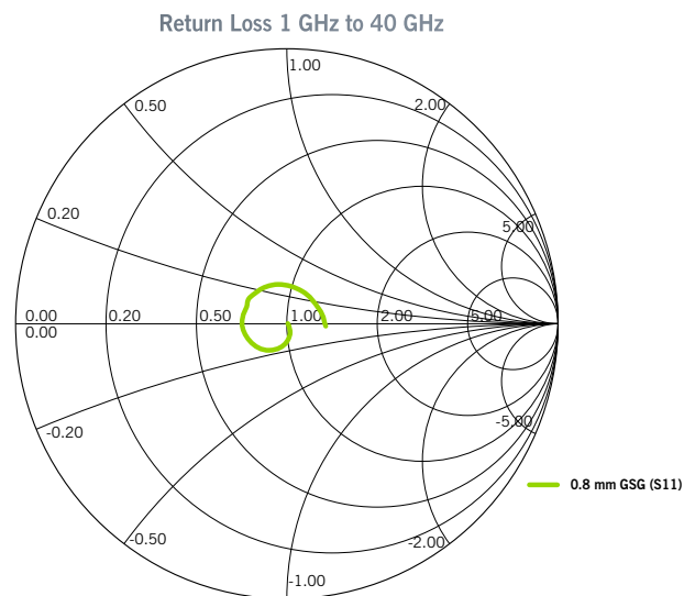
Figure 10. GSG P8A Return Loss plotted on Smith chart, 0.8 mm pitch
