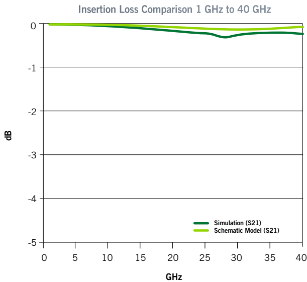
Figure 12. GSG P8A Insertion Loss, 0.8 mm pitch
