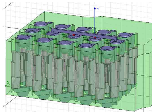
Figure 15. 0.8 mm GSSG model configuration
