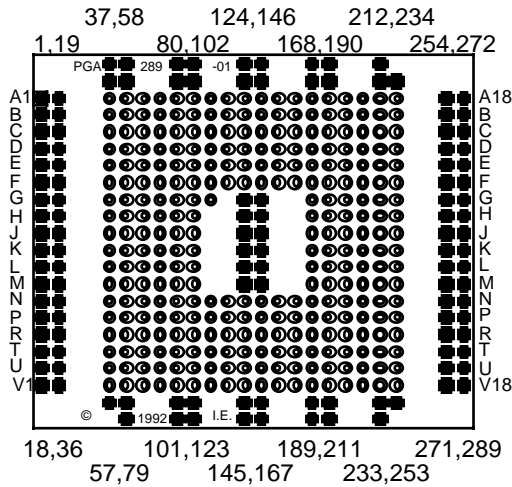
Top View- PGA
