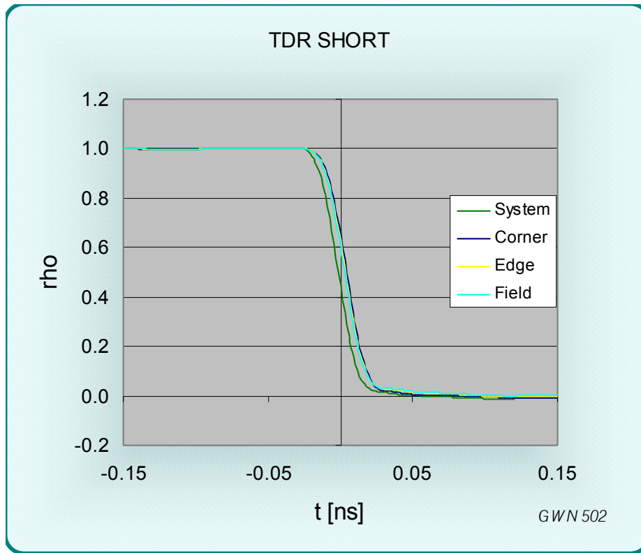
Figure 6 TDR signal from a SHORT circuited SM interposer
