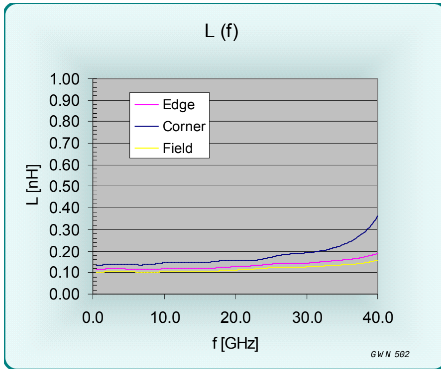
Figure 15 L(f) for the SM interposer
