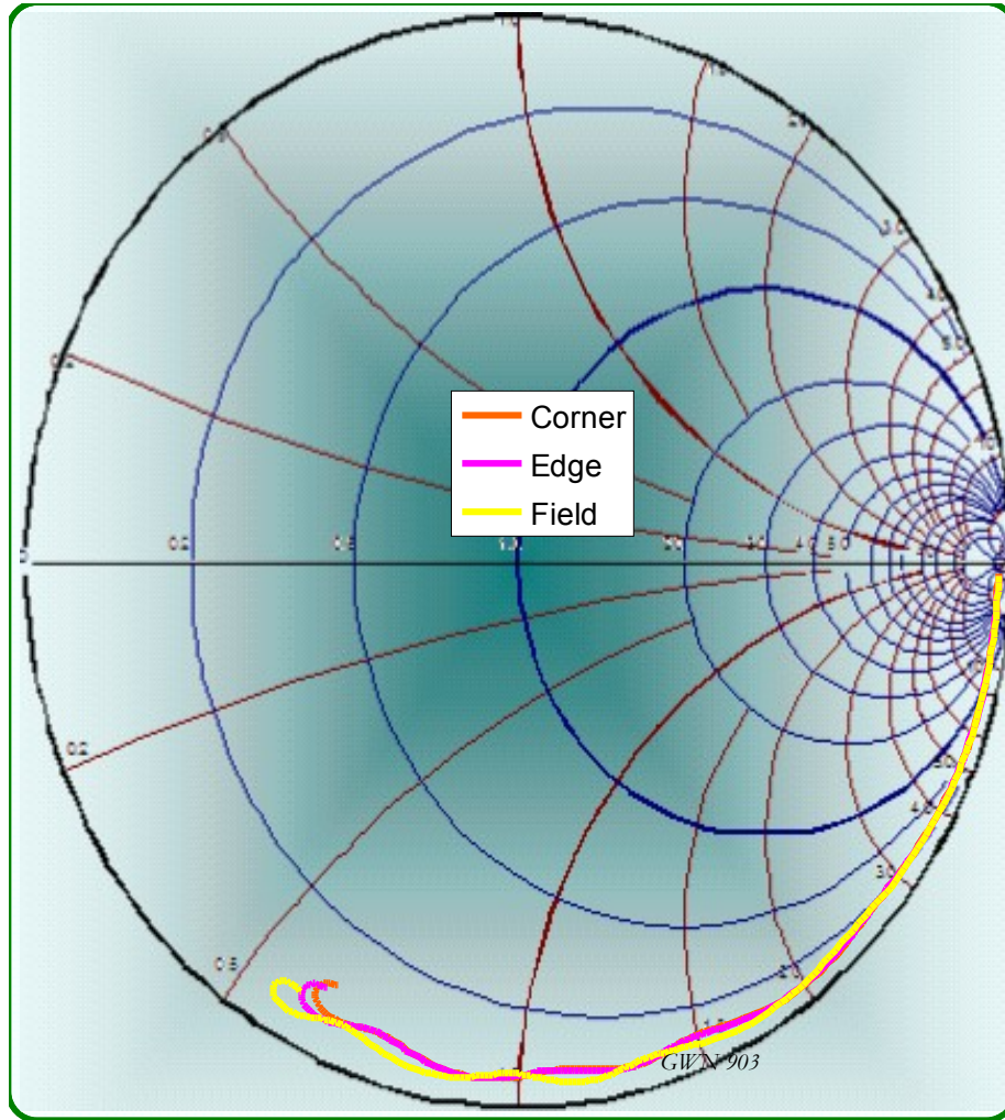
Figure 12 Reflections from the open circuited SM interposer
