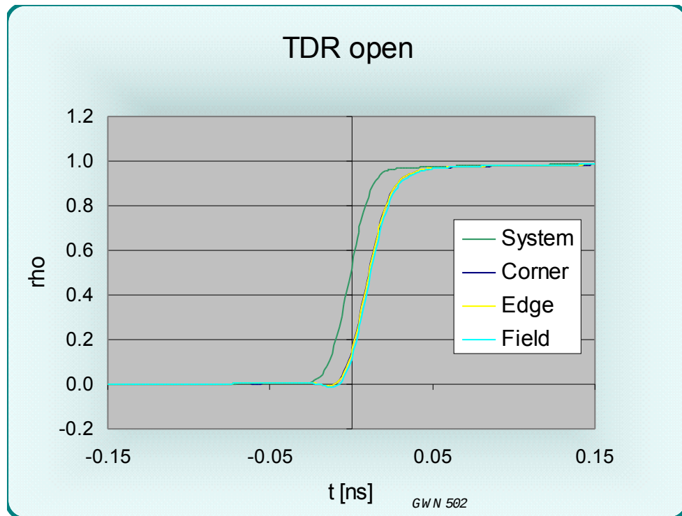
Figure 5 TDR signal from an OPEN circuited SM interposer
