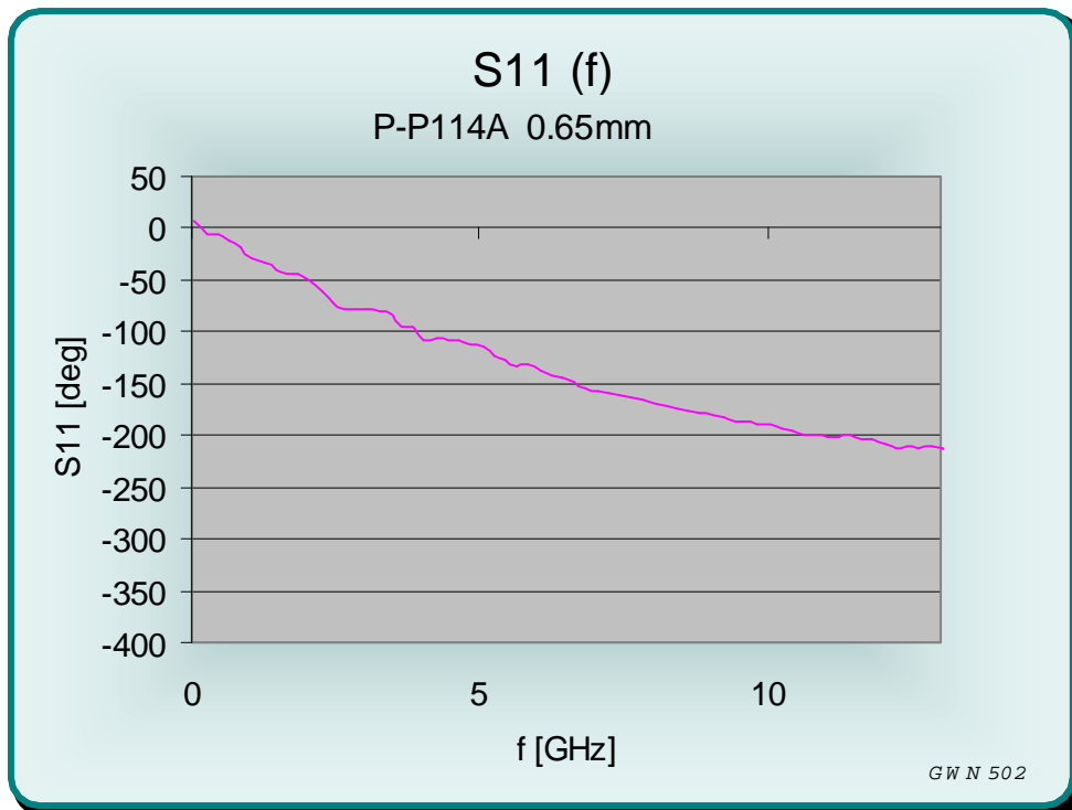
Fig. 3 S11 (f) for the open circuited signal pin
